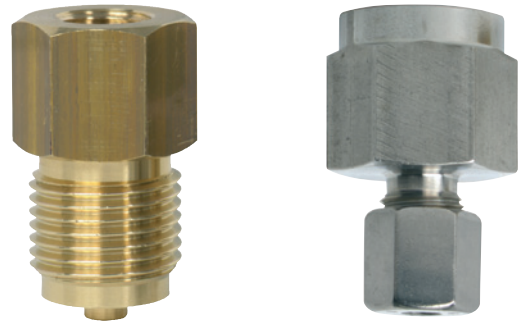
Fig. left: Adapter, male-female, G ½ / G ¼ B
